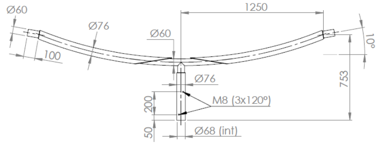
ITO DOUBLE S1250
