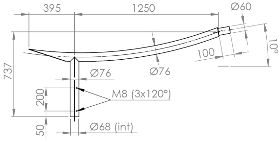
ITO SIMPLE S1250
