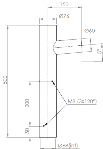
ITO SIMPLE S150
